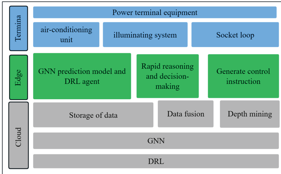
Figure 1 "Cloud-edge-end" three-tier system architecture
