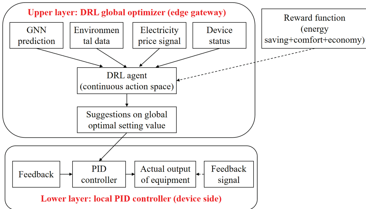
Figure 2 Double-layer DRL intelligent control architecture
