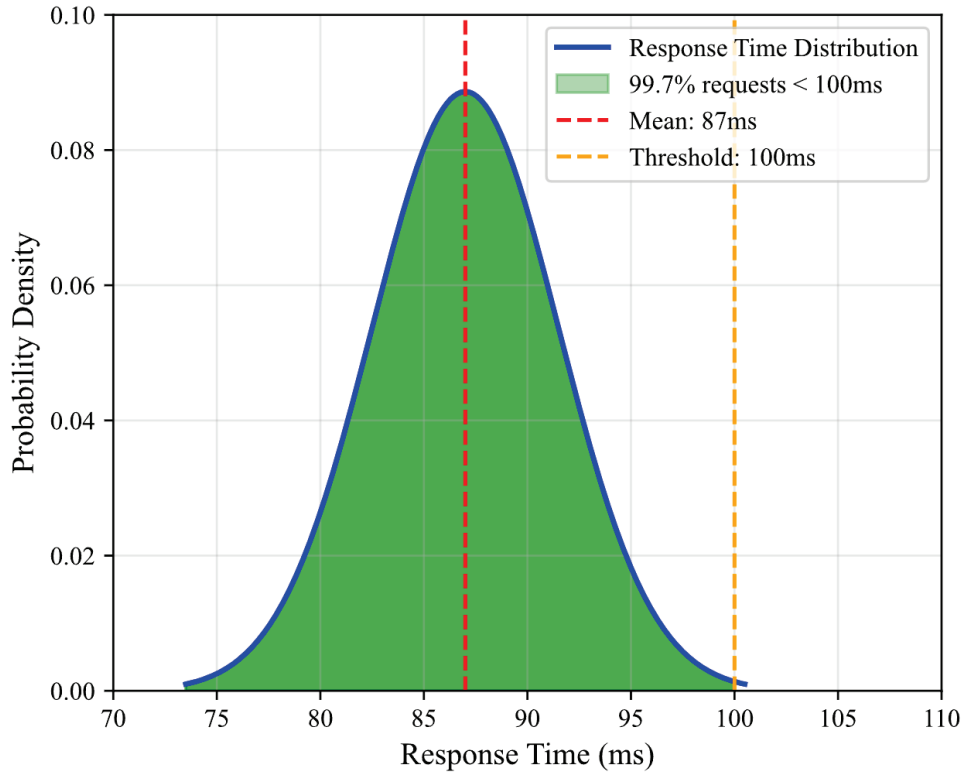
Figure 4 Decision response time distribution of edge gateway
